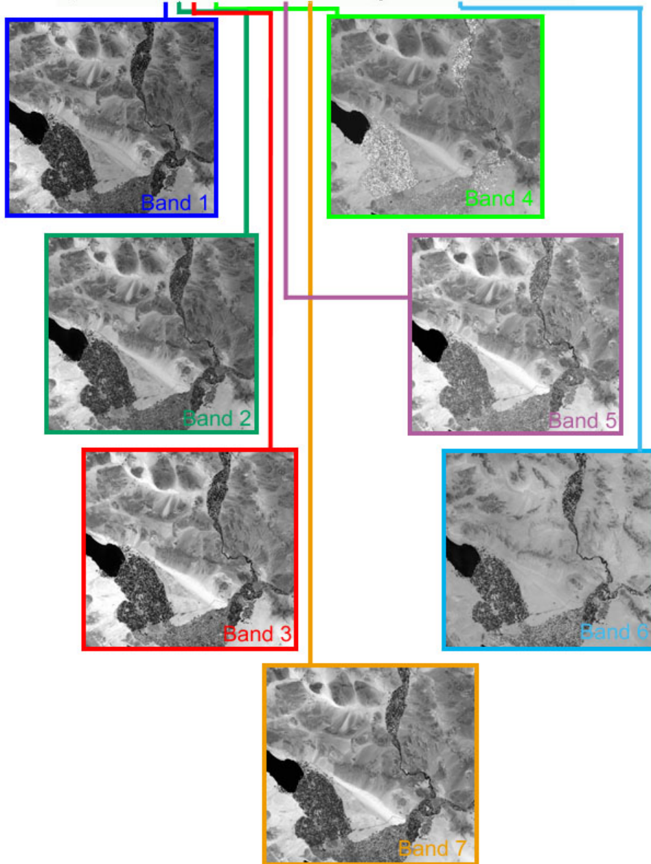
Electromagnetic Spectrum Image from Virtual Hawaii .
