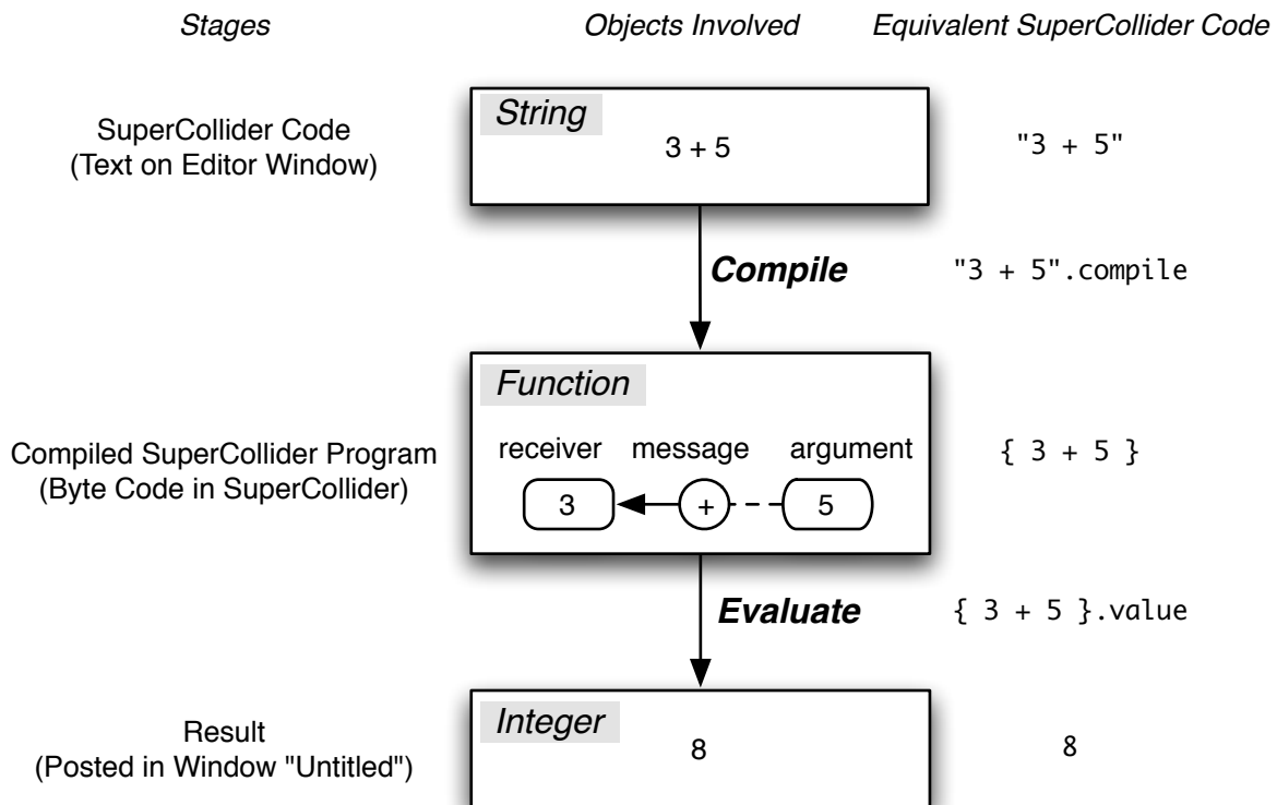
Figure (n) Compiling and Evaluating Code
